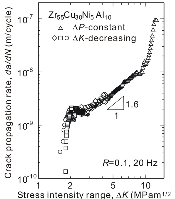
Fig. 1. Crack propagation behavior.
